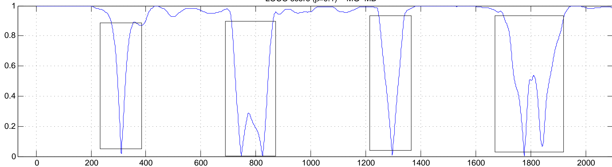
LOCO score ( \beta=0.1 ) – MG–MD
