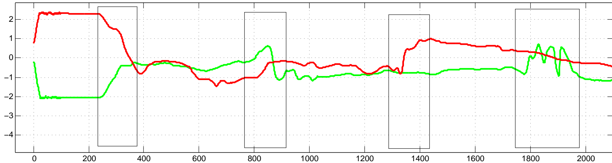
Normalized MD and MG angles
